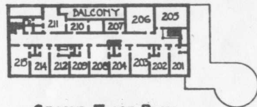
SECOND FLOOR PLAN ANNEX
